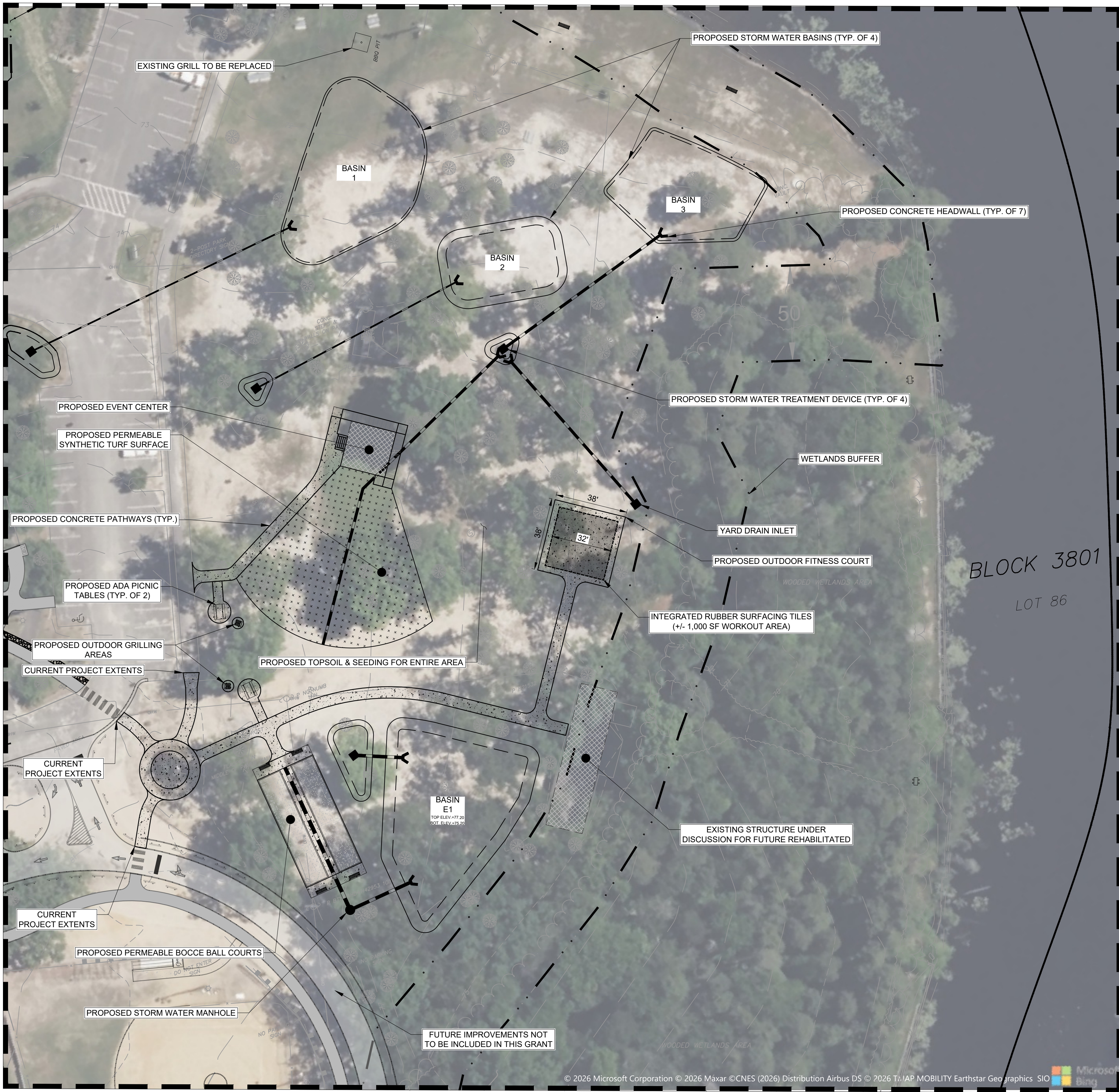
INSET 2 - RECREATIONAL DEVELOPMENT & IMPROVEMENTS SCALE 1" = 30'
